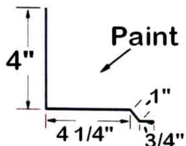
Universal Endwall
