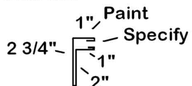
F Channel
