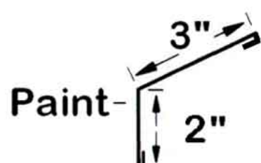
Fascia #1
