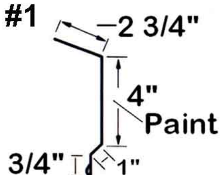
Universal Sidewall
